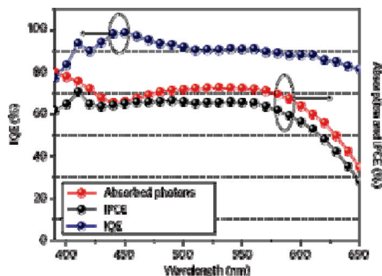
Figure 34. Internal quantum efficiency (IQE) of P81b:PC 71 BM solar cells. (a) IQE values of the 1:4 device with film cast from DCB. The red line shows the total absorption of the device, and the black line the IPCE. Adapted with permission from ref 132. Copyright 2009 Nature Publishing Group.
